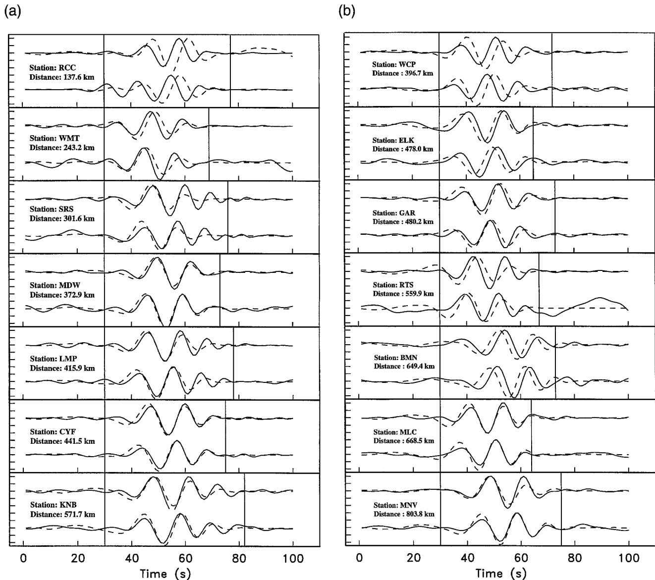
Figure 2. (a) The vertical- and radial-component seismograms used in this study to estimate Colorado plateau crustal structure. The solid lines show the recorded seismograms that have been instrument deconvolved to displacement and bandpass filtered between periods 10, and 50 sec. For each station, the upper traces are from vertical-component seismograms, and the lower trace is radial component. The vertical lines indicate the portion of the seismograms used for waveform fitting, and the source-to-receiver distance is shown for each station. Each of the seismograms are normalized to their maximum amplitudes. The dashed lines show the synthetic waveforms predicted by our best-fitting one-dimensional crustal model for this region. Note that the recorded seismograms are slightly slower than those predicted by our model for stations CYF, LMP, and SRS and faster for stations WMT and RCC. (b) Similar to Figure 2a, but for stations used in modeling the crustal structure of the Great Basin province. We note that the seismograms recorded at stations BMN and ELK are slightly slower and seismograms at WCP and RTS are slightly faster than those predicted by our average model.
