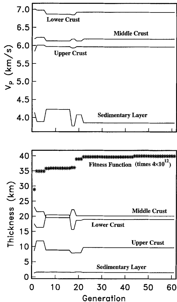
Figure 5. P -wave velocity, thickness, and wave-form fitness as a function of generation number for a genetic algorithm run with noise-free data (described in text). The crustal model that best fits the synthetic seismograms for an input model (Fig. 7) is plotted for each generation. We note that adequate convergence is reached by the 25th iteration. A one-point crossover scheme is adopted for this run with the crossover probability equal to 0.85 and the mutation probability equal to 0.125 (described in text).
