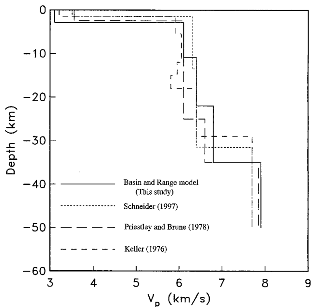
Figure 8. Comparison between our final Great Basin model with several published models of one-dimensional crustal structure of the region. Compared to others, our model shows a slightly thicker sedimentary layer and higher lower crustal velocity. We do not require the crustal low-velocity zone as reported by Keller et al. (1976). Uncertainties in our preferred model are given in Table 2.
