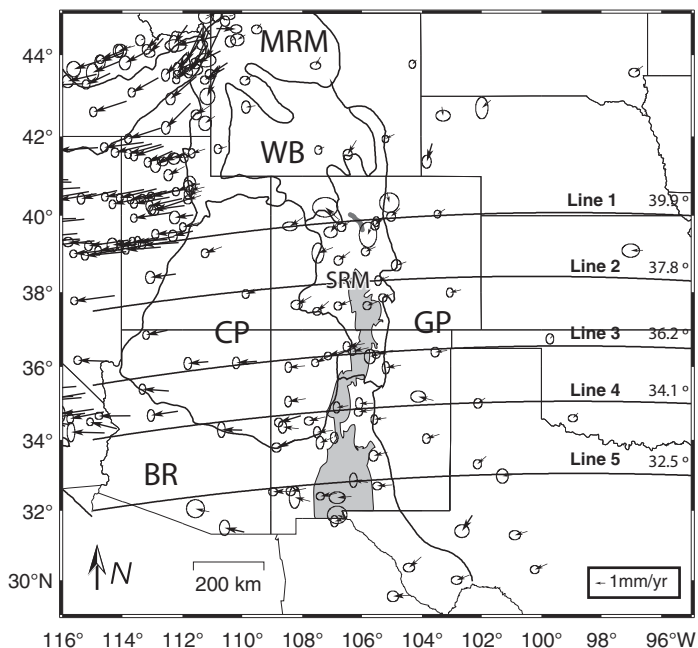
Figure 2. Locations of profile lines as numbered; west end of each profile line is the left side of Figure 3. Arrows indicate the direction and magnitude of GPS velocity estimates. Ellipses are 95% confidence. Thick black lines denote major physiographic boundaries (Fenneman and Johnson, 1946): MRM—middle Rocky Mountains, WB—Wyoming Basin, SRM—southern Rocky Mountains, CP—Colorado Plateau, GP—Great Plains, BR—Basin and Range. Light gray lines indicate state boundaries. Latitude at which each profile passes through 109°W is labeled on the right. Gray shaded region in Colorado and New Mexico indicates the rough extent of Rio Grande Rift basins. Williams Fork Mountains fault in north-central Colorado is indicated with a thick gray trace.
