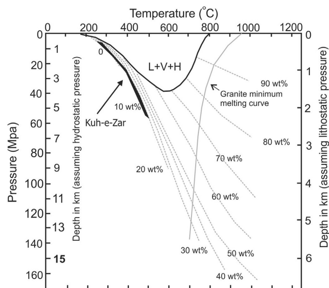
Fig. 19. Pressure-temperature diagram showing phase relationships in the NaCl-H 2 O system at lithostatic and hydrostatic pressures (Fournier, 1999). L = liquid, V = vapor, H = halite. Thin dashed lines are contours of constant wt percent NaCl dissolved in brine. Filled gray line indicates granite minimum melting curve. Filled dark line shows the three-phase boundary, L + V + H, for the system NaCl-KCl-H 2 O with Na/K in solution fixed by equilibration with albite and K-feldspar at the indicated temperatures. Location of Kuh-e-Zar fluid inclusions data plotted on it.
