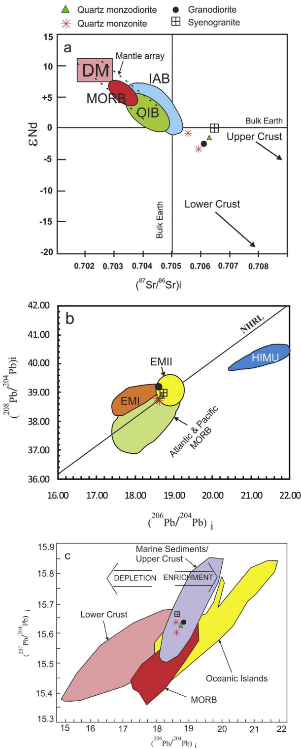
Fig. 14. Plots of Sr–Nd–Pb isotopic compositions for the Kuh-e-Zar intrusive rocks. a) (^{87}\text{Sr}/^{86}\text{Sr})_i versus \epsilon_{\text{Nd}} ; b) (^{208}\text{Pb}/^{204}\text{Pb})_i versus (^{206}\text{Pb}/^{204}\text{Pb})_i ; c) (^{207}\text{Pb}/^{204}\text{Pb})_i versus (^{206}\text{Pb}/^{204}\text{Pb})_i . MORB: Mid ocean ridge basalts; DM: Depleted mantle; OIB: Ocean-island basalts; IAB: island arc basalts; EM I and II: enriched mantle reservoirs; NHRL: Northern Hemisphere Reference line; HIMU: high U/Pb mantle (e.g., Zindler and Hart, 1986; Rollinson, 1993; Wang et al., 2006). Initial ratios calculated for 41 Ma. Pb isotope ratios in major terrestrial reservoirs are from White (2003) and references therein.
