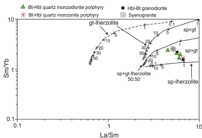
Fig. 18. Plot of Kuh-e-Zar intrusives on Sm/Yb vs. La/Sm diagram for determination of magma source. (Modified after Aldanmaz et al. (2000).)
