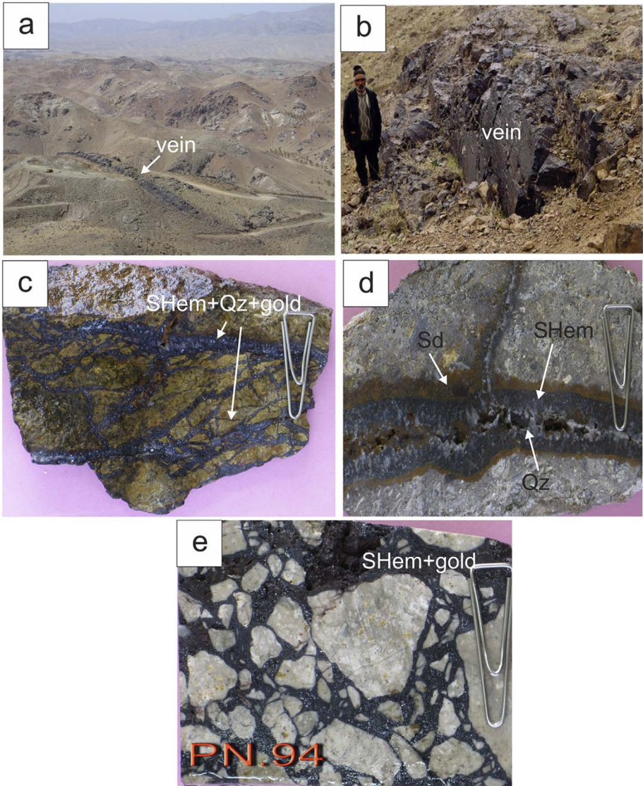
Fig. 6. a. Vein-type mineralization in fault zone at Mohammad Baigi mineralized zone (looking to NW). b. Specular hematite-gold-quartz vein in Tangeh Piaz mineralized zone. c. Stockwork-like texture bearing specular hematite-quartz-gold veinlets. d. Open space filling texture in the veinlet ores. e. Hydrothermal breccia consists of brecciated fragments of the altered host rock cemented by specular hematite and gold. (Qz: quartz, SHem: specular hematite, Sd: siderite (Whitney and Evans, 2010).)
