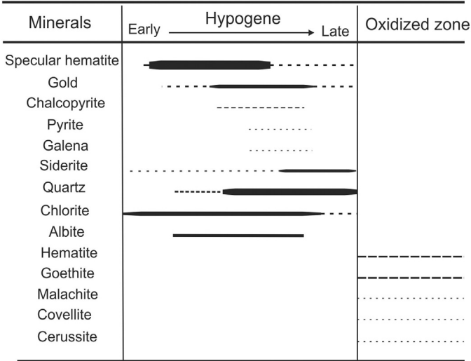
Fig. 7. Paragenetic sequence of mineral assemblages in the Kuh-e-Zar deposit.
