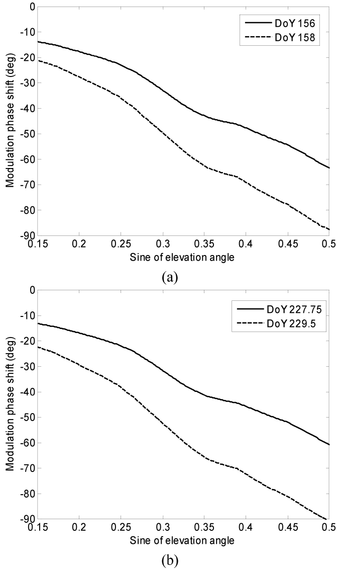
Fig. 9. Phase \Psi(\theta) calculated for soil moisture profiles measured on (a) DoY 156 and DoY 158, and on (b) DoY 227.75 and DoY 229.5.
