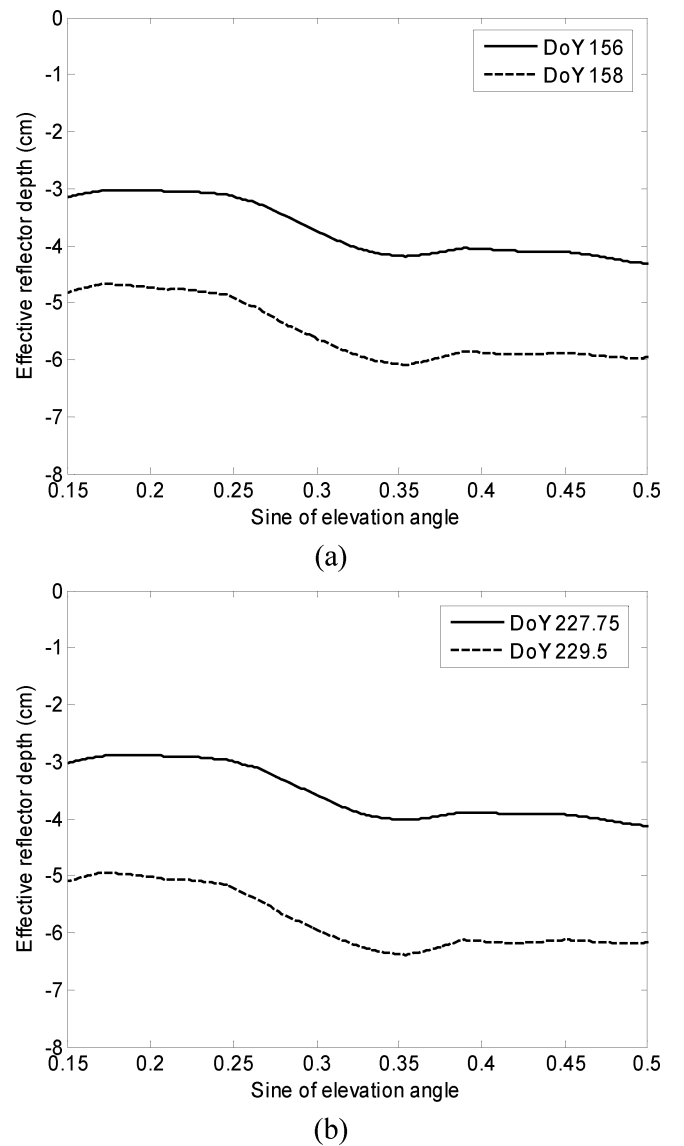
Fig. 10. Effective reflector depth \Delta h(\theta) calculated for soil moisture profiles measured on (a) DoY 156 and DoY 158, and on (b) DoY 227.75 and DoY 229.5.
