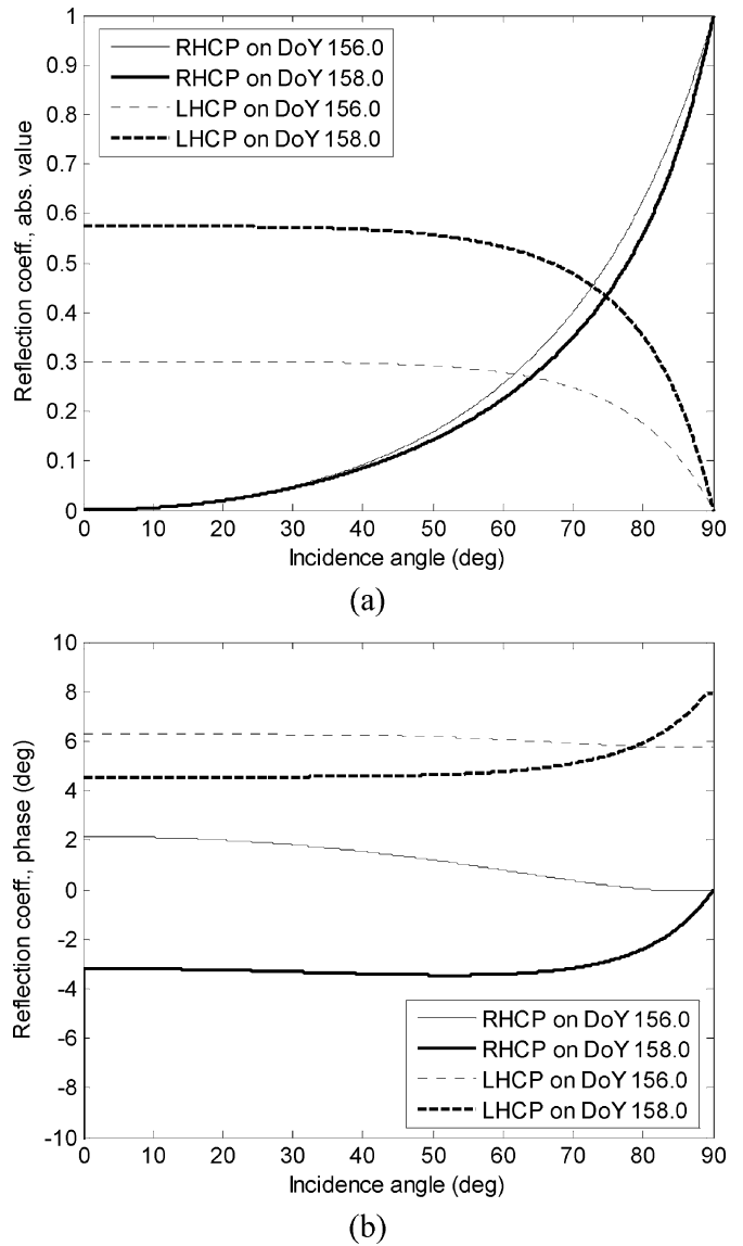
Fig. 5. Reflection coefficients at two circular polarizations for the cases of the profile shown in Fig. 4(a) and (b); (a) corresponds to amplitude and (b) to phase of the reflection coefficient.
